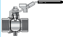
BVG4PLOCK BSSP, Vented & Locking Handle P. 95
